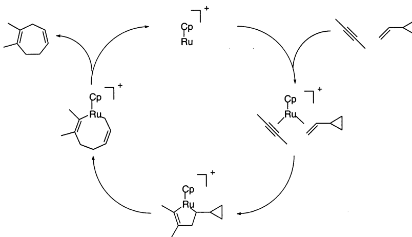
Scheme 7. A [5+2] Cycloaddition
